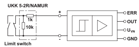
Application drawing
