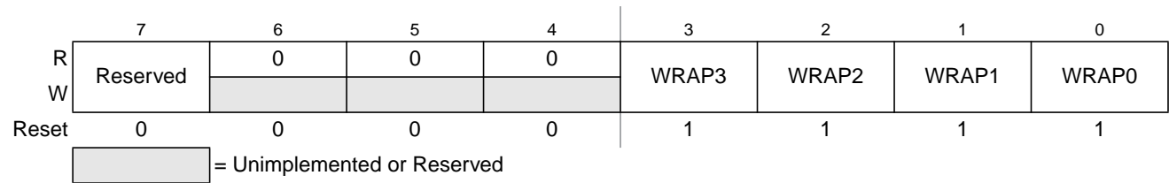
Figure 10-3. ATD Control Register 0 (ATDCTL0)
