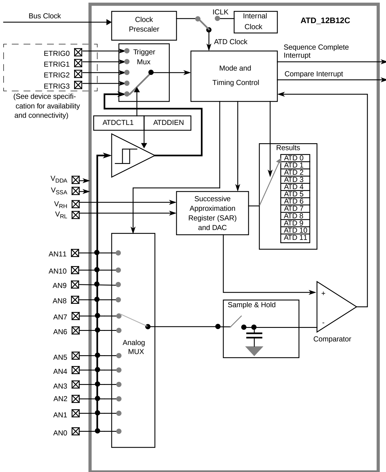
Figure 10-1. ADC12B12C Block Diagram
