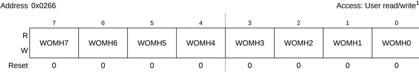
Figure 2-50. Port H Wired-Or Mode Register (WOMH)
