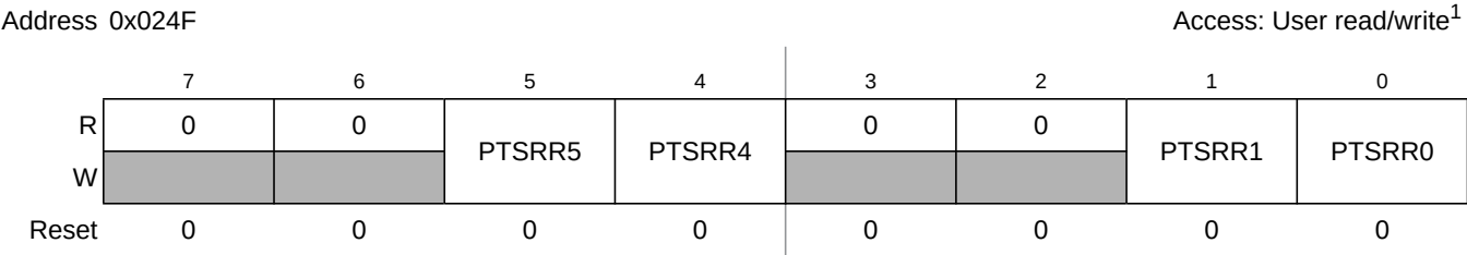
Figure 2-27. Port S Routing Register (PTSRR)
