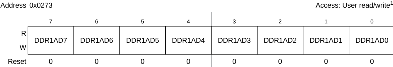
Figure 2-56. Port AD Data Direction Register (DDR1AD)
