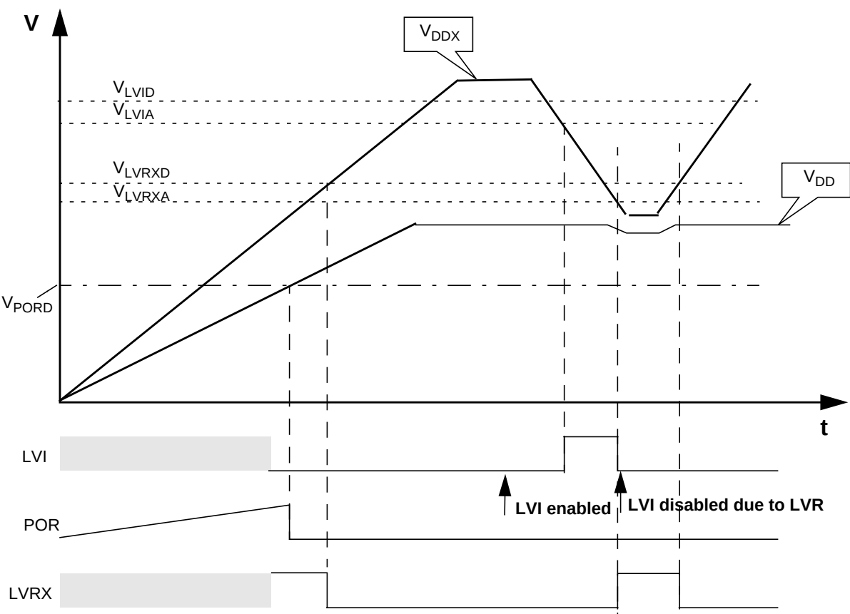
Figure A-2. 9S12XHY family - Chip Power-up and Voltage Drops (not scaled)
