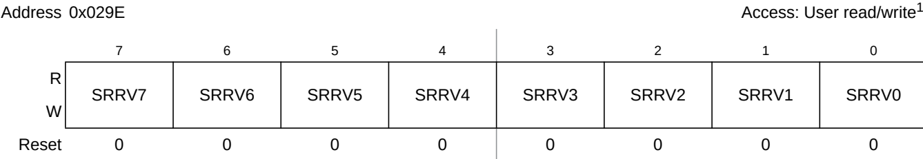
Figure 2-92. Port V Polarity Select Register (SRRV)
