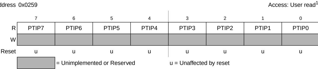
Figure 2-37. Port P Input Register (PTIP)
