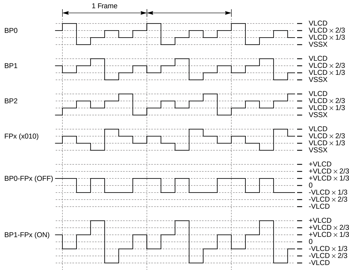
Figure 17-13. 1/3 Duty and 1/3 Bias
