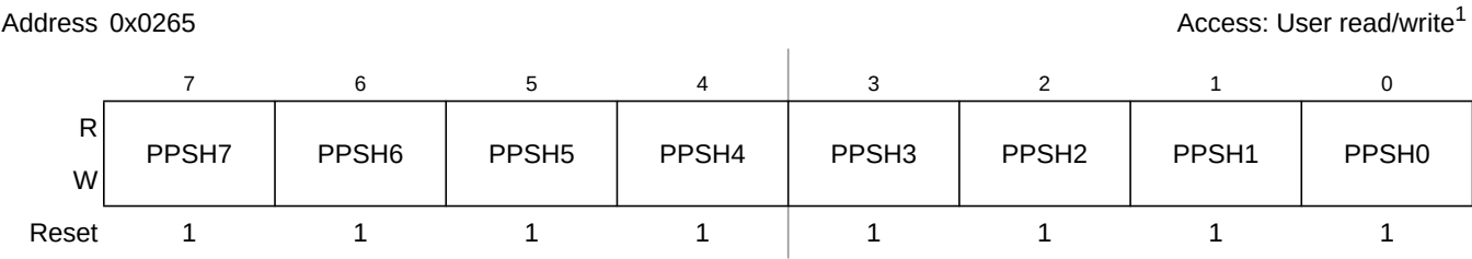
Figure 2-49. Port H Polarity Select Register (PPSH)
