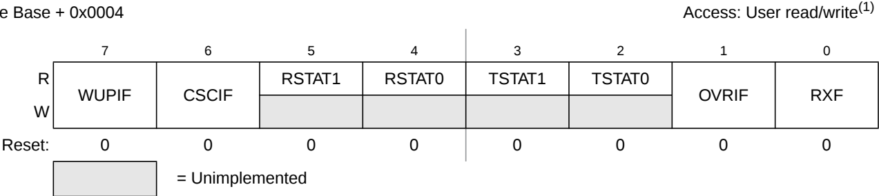
Figure 11-8. MSCAN Receiver Flag Register (CANRFLG)
