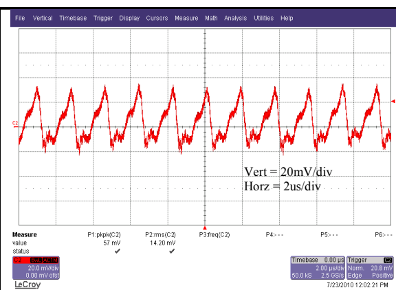
Vo=1.8V Typical Input Ripple at nominal Input Voltage and full load at Ta=25 degrees. Input capacitors 4 x 22uF ceramic
