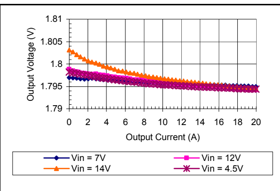
Vo=1.8V Typical load regulation
