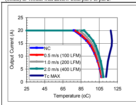
Vo=0.7V, Vin=12V maximum output current vs. ambient temperature at nominal input voltage for natural convection (60lfm) to 400lfm with airflow from pin 3 to pin 2.
