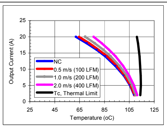
Vo=3.3V, Vin=12V maximum output current vs. ambient temperature at nominal input voltage for natural convection (60lfm) to 400lfm with airflow from pin 3 to pin 2.
