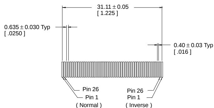
Detail A
