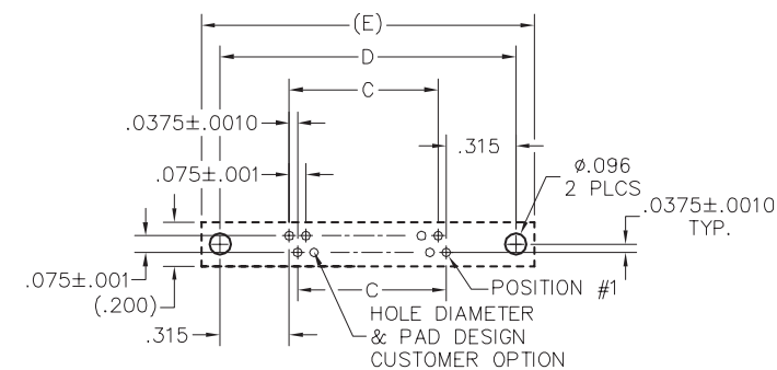
PCB LAYOUT VIEWED FROM COMPONENT SIDE
