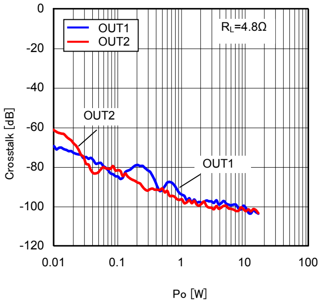
Figure 43. Crosstalk vs P_o (4.8 \Omega )
