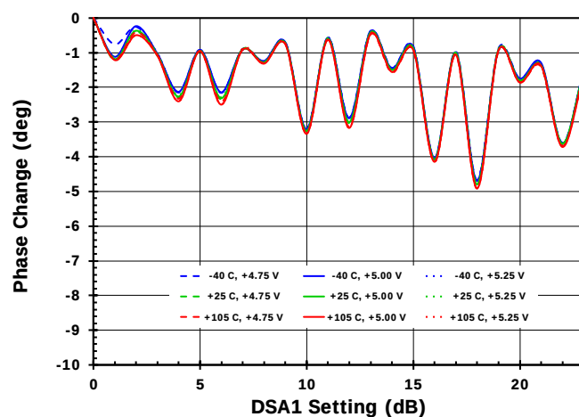
Figure 16. Phase Deviation Between Adjacent States vs. DSA1 Setting
