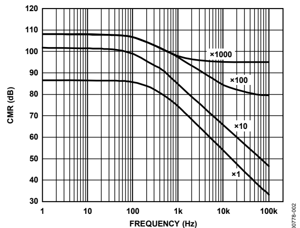
Figure 2. CMR vs. Frequency, 5 V S , 0 V O
