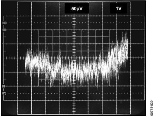
Figure 39. Gain Nonlinearity, G = -100 , 15\text{ ppm/DIV}
