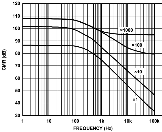
Figure 17. CMR vs. Frequency, V_S = 5V_S, 0V_S, V_{REF} = 2.5V
