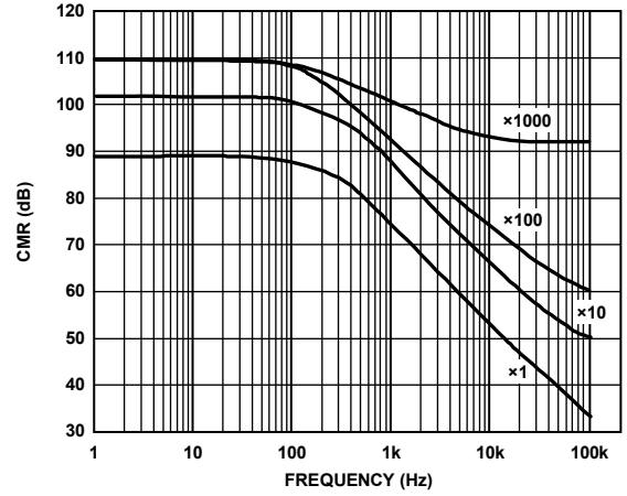
Figure 18. CMR vs. Frequency, \pm 5V_S
