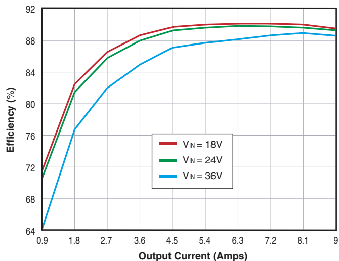
UWR-3.3/9-D48 Efficiency vs. Load @ 25°C Ambient
