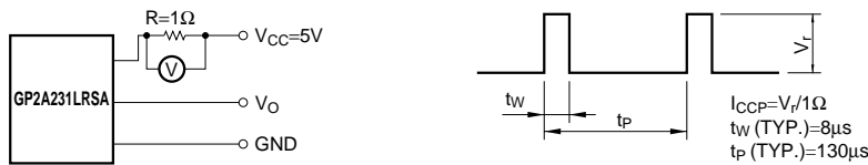
Fig.1 Test Condition for Peak Pulse Value I_{CCP}
