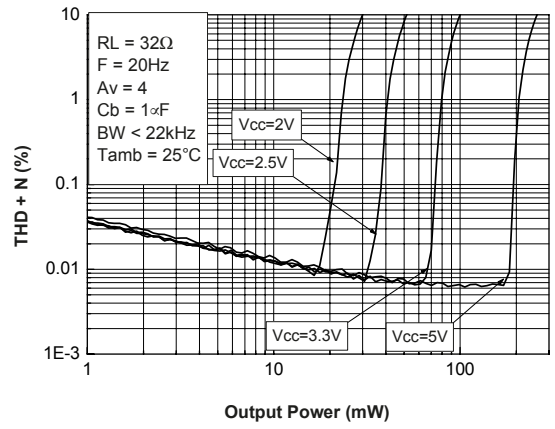
Figure 58. THD + N vs. output power RL = 32 Ω
