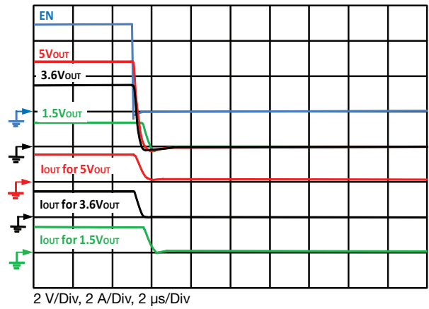
Figure 22 - Typical Fall Time C_{OUT} = 0.1 \mu F , C_{IN} = 4.7 \mu F , I_{OUT} = 1.5 A
