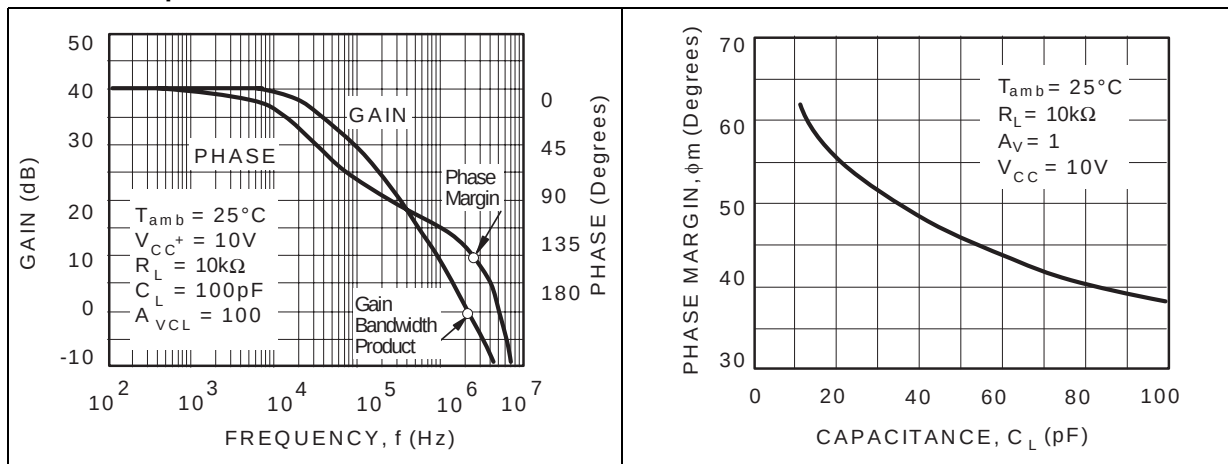
Figure 9. Open loop frequency response and phase shift Figure 10. Phase margin vs. capacitive load
