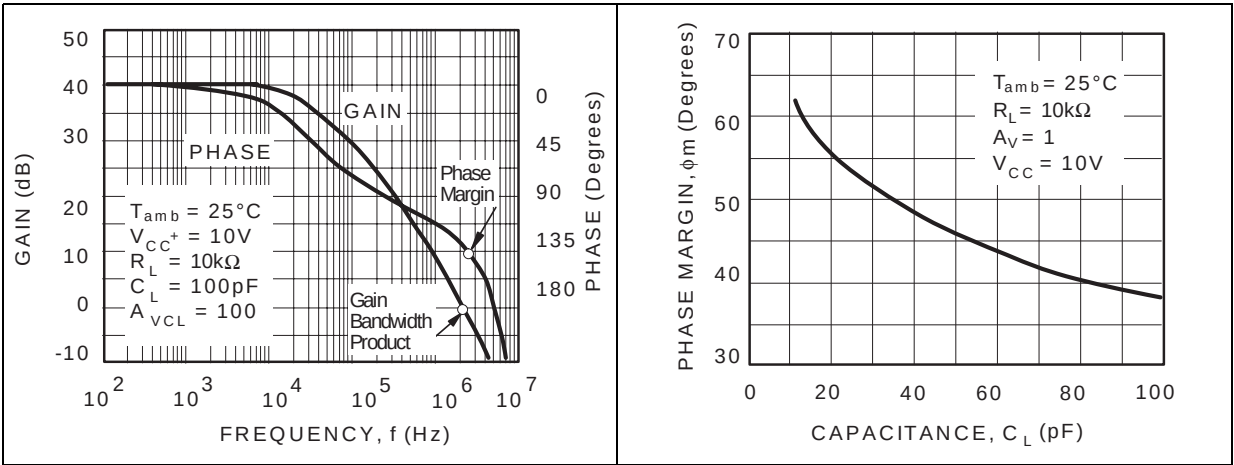
Figure 9. Open loop frequency response and phase shift Figure 10. Phase margin vs. capacitive load
