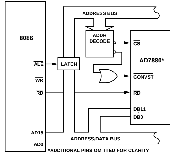
Figure 19. AD7880–8086 Interface
