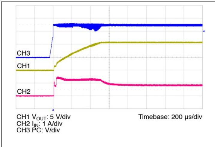
Figure 10 — Start up from application of PC; V_{IN} pre-applied C_{OUT} = 1200 \mu F
