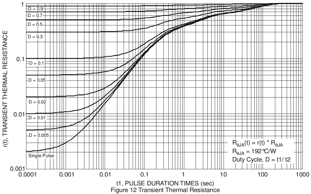
t_1 , PULSE DURATION TIMES (sec) Figure 12 Transient Thermal Resistance
