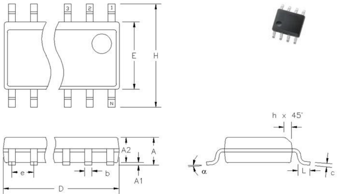
Figure 10: Package drawing
