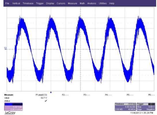
Figure 16. 264 V / 50 Hz
