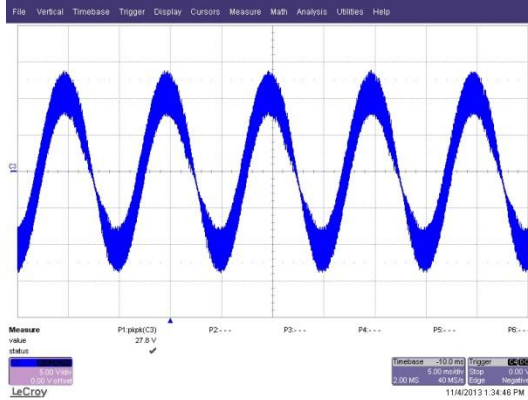
Figure 15. 180 V / 50 Hz
