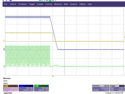
Figure 14. PFC OFF
