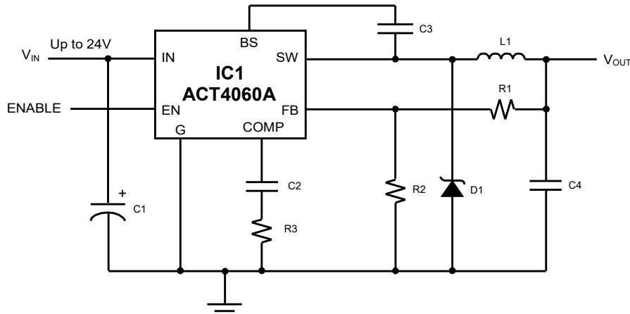
Figure 5: ACT4060A 5V/2A Output Application ①
