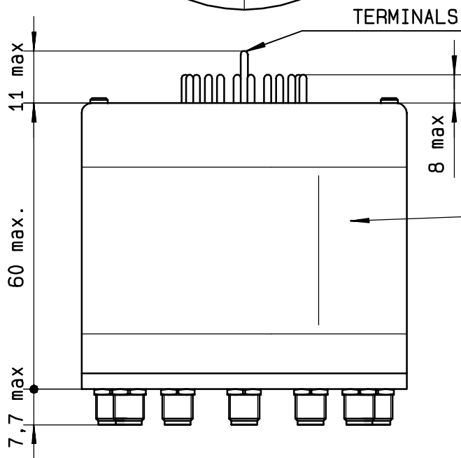
TOP VIEW (TERMINALS)
