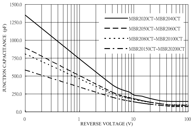
FIG. 4-TYPICAL JUNCTION CAPACITANCE
