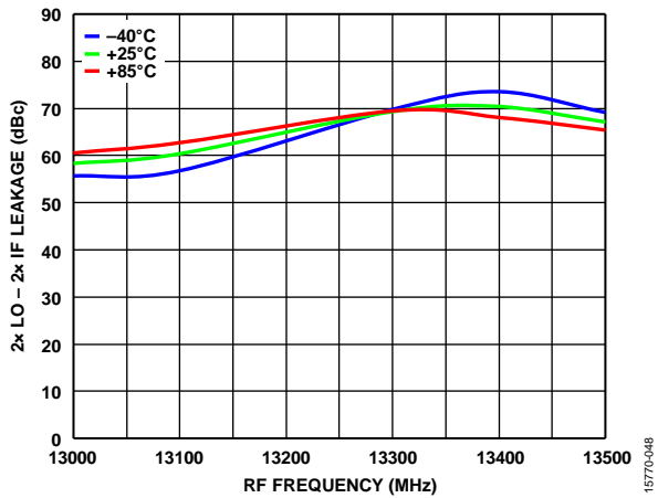
Figure 48. 2\times\text{LO} - 2\times\text{IF} Leakage vs. RF Frequency at Various Temperatures, \text{IF} = 3.3\text{ GHz} , -10\text{ dBm}
