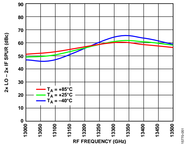
Figure 51. 2\times\text{LO} - 2\times\text{IF} Leakage vs. RF Frequency at Various Temperatures, \text{IF} = 3.3\text{ GHz} , 0\text{ dBm}
