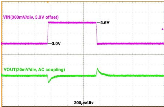
Figure 22. Line Transient, V_{IN} = 3.0\text{ V} \Leftrightarrow 3.6\text{ V} , V_{OUT} = 1.8\text{ V} , 10\text{ }\mu\text{s} Edge, 300\text{ mA} Load, Auto Mode
