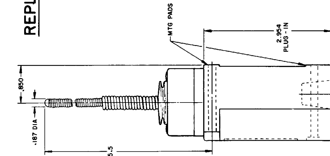
PLASTIC EXTENSION TYPE 7A ACTUATOR TYPE LSJ1 AND LSJ3
