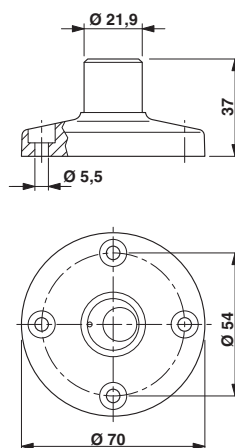
Dimensioned drawing
