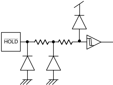
Figure 55. HOLD input equivalent circuit
