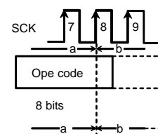
Figure 46. WREN/WRDI cancel valid timing
