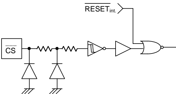
Figure 52. CS input equivalent circuit
