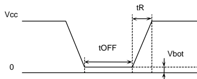
Figure 58. Rise waveform
