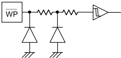
Figure 56. WP input equivalent circuit
