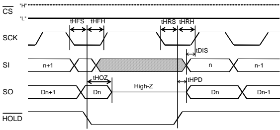
Figure 3. HOLD timing
