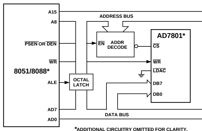
Figure 31. AD7801–8051/8088 Interface
