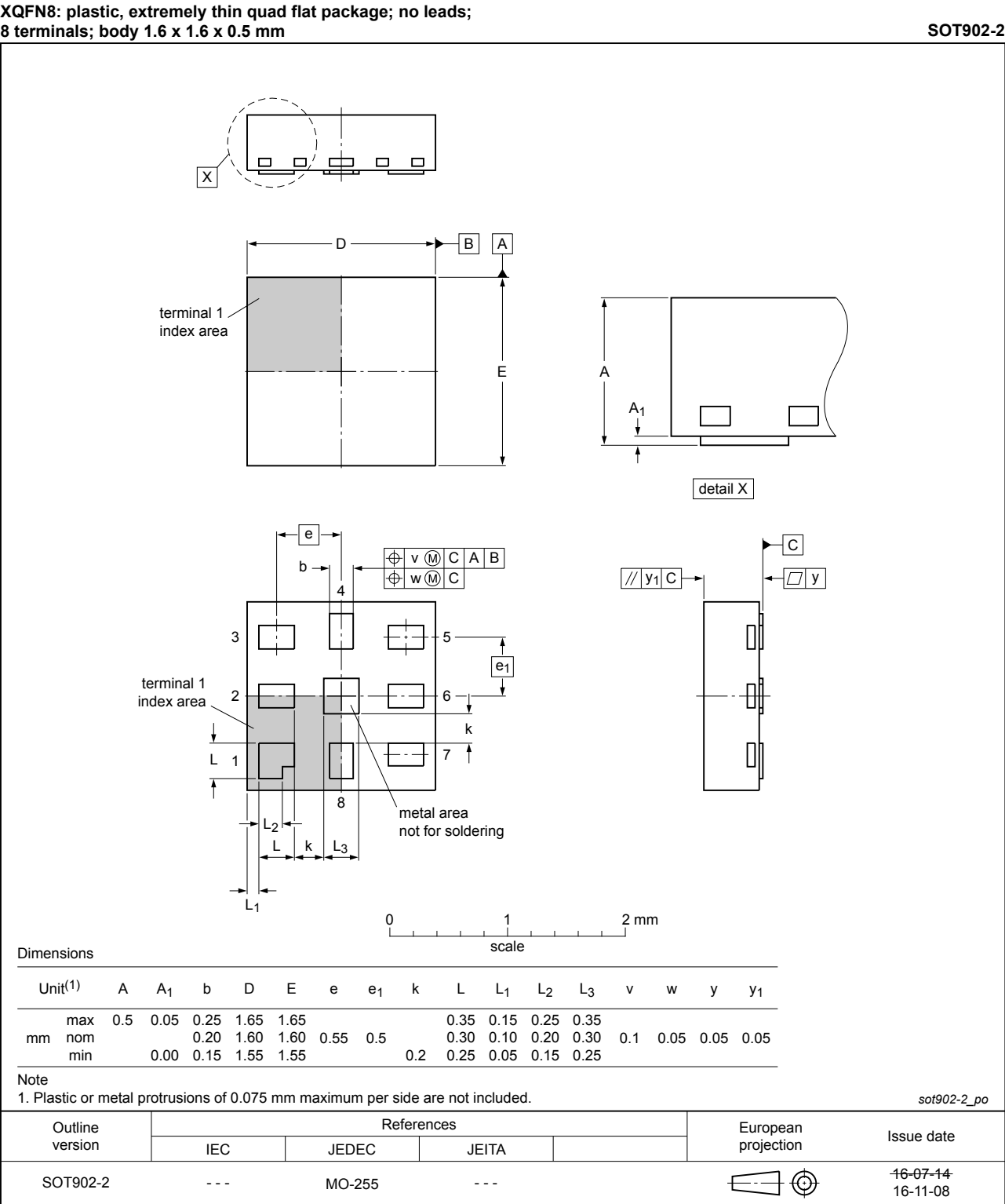
Figure 13. Package outline SOT902-2 (XQFN8)
