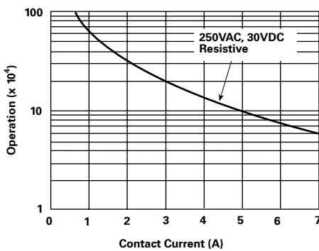
Electrical endurance
