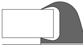
Too much solder Pad geometry too large KKE0071-A-E
