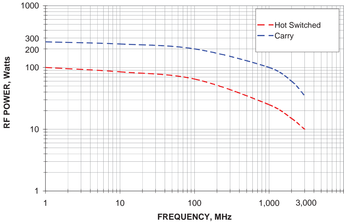
RF255/RF257 RF POWER HANDLING CAPABILITY
