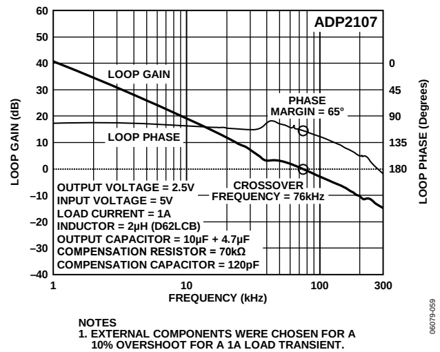
Figure 45. ADP2107 Bode Plot at V_{IN} = 5V , V_{OUT} = 2.5V and Load = 1 A
