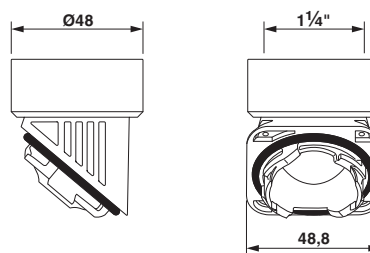
Dimensional drawing
