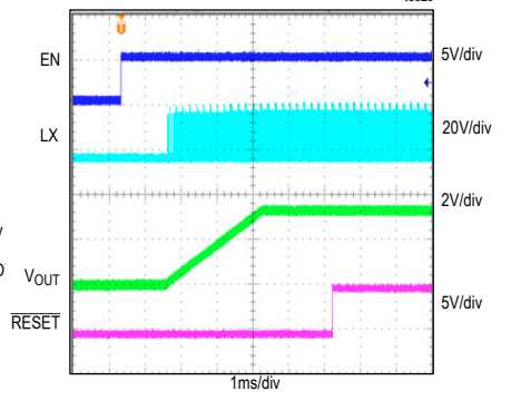
STARTUP THROUGH ENABLE
