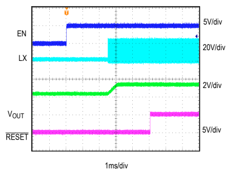
STARTUP WITH 2.5V PREBIAS
