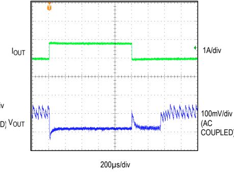
LOAD CURRENT TRANSIENT RESPONSE
