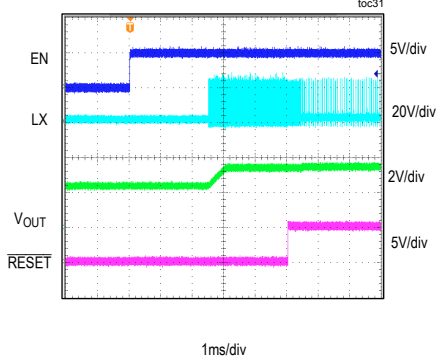
STARTUP WITH 2.5V PREBIAS
