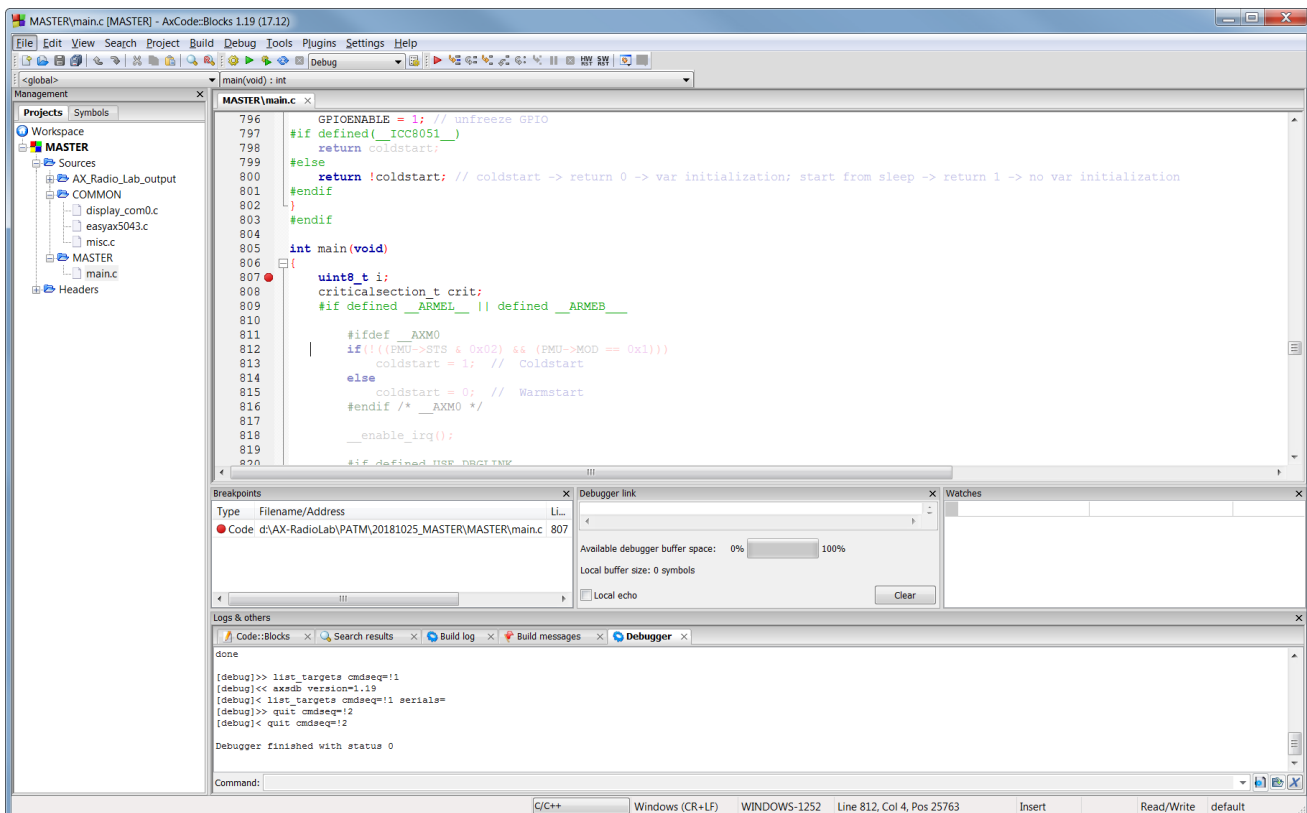
Figure 16. AxCode::Blocks
