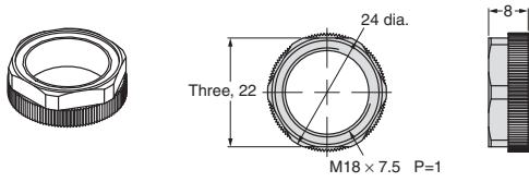
For E3FA/E3RA
