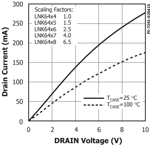
Figure 15. Output Characteristic.
