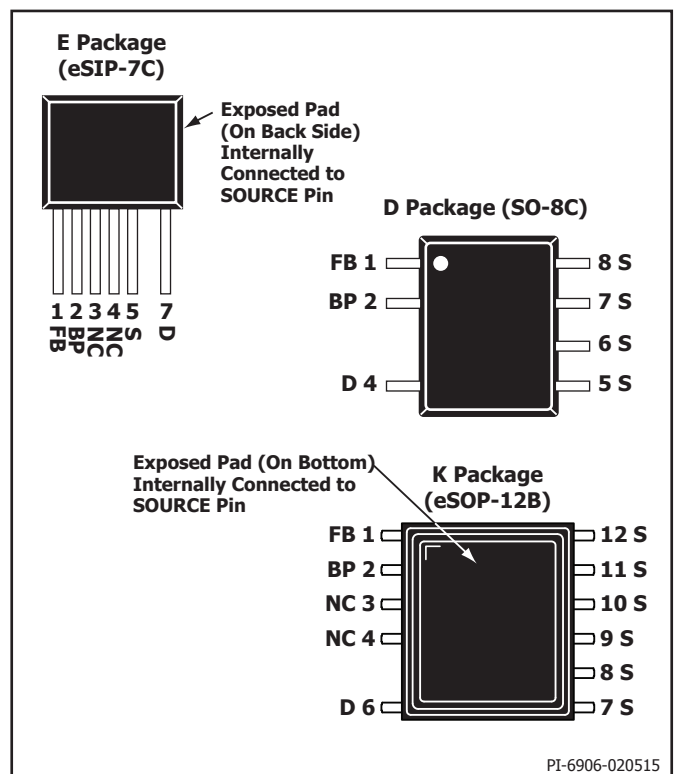
Figure 3. Pin Configuration.
