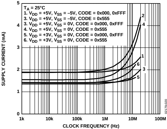
Figure 20. AD7398 Supply Current vs. Clock Frequency
