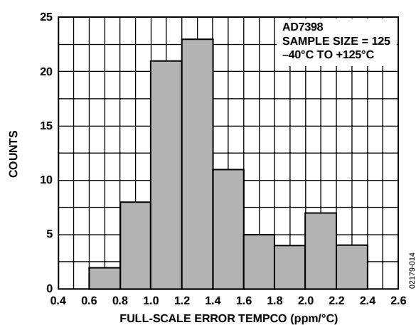
Figure 14. AD7398 Full-Scale Error Tempco
