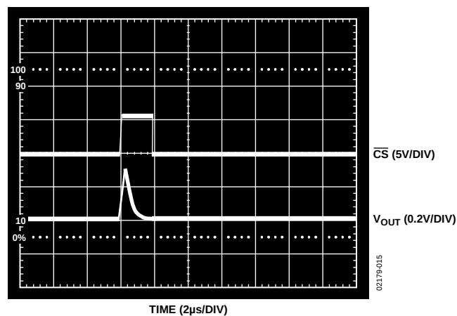
Figure 15. AD7398 Midscale Glitch
