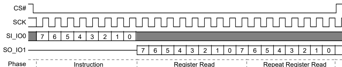
Figure 113. PPB Lock Register Command Sequence
