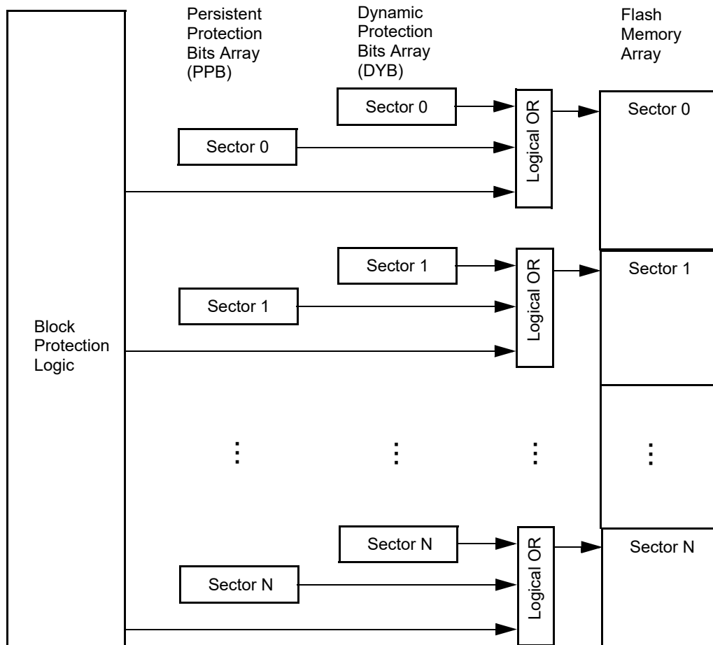
Figure 43. Sector Protection Control
