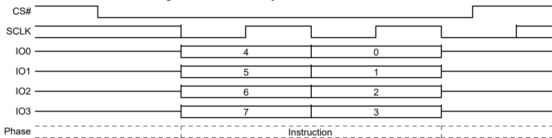
Figure 71. Enter 4 Byte Address QPI Mode
